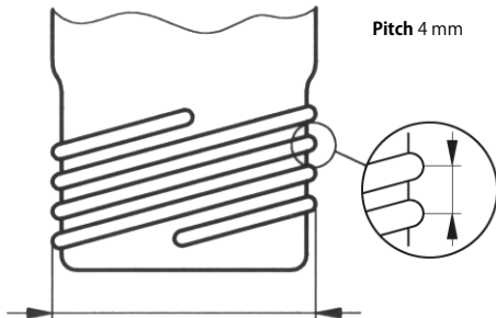
GL 32 – outer-Ø = 32 mm
