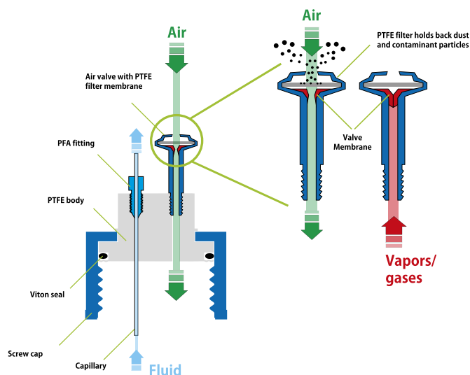
Figure 1 Working principle of a safety cap with an air inlet valve. When the liquid is drawn off, air can flow in. Evaporation of the liquid is prevented by a valve membrane.
