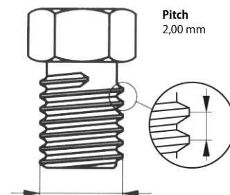
M 16 – outer- \varnothing = 16 mm
