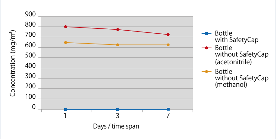
Fig. 3 Methanol emissions and acetonitrile emissions in the test chamber.
