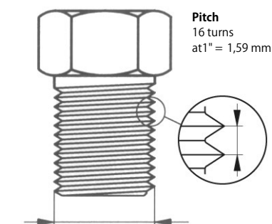
UNF 3/4"-16G – outer- \varnothing = 18,9 mm
