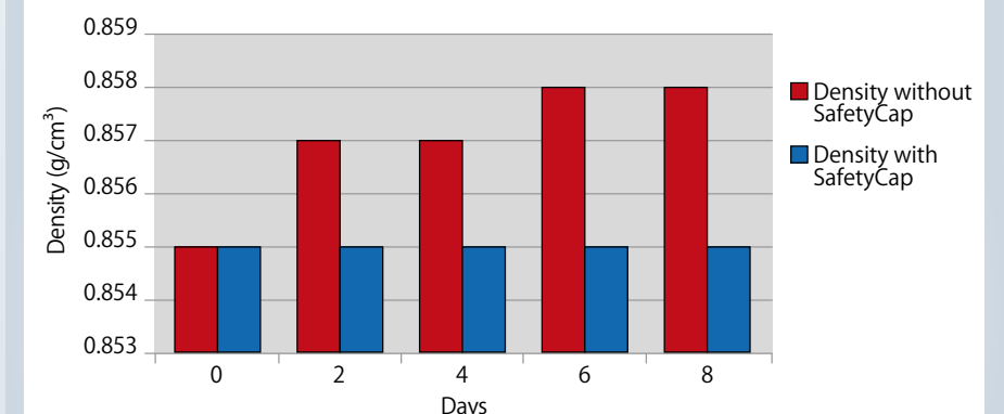
Fig. 1 Changes in the density of a methanol/water mixture
