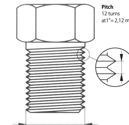
UNF 1"-12G – outer- \varnothing = 25,2 mm
