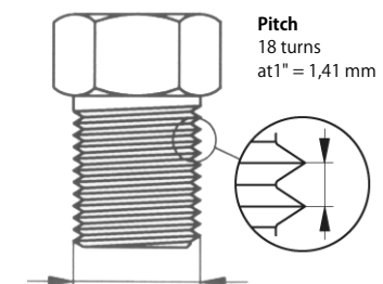
UNF 5/8"-18G – outer- \varnothing = 15,7 mm
