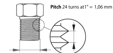
UNF 3/8"-28G – outer- \varnothing = 9,4 mm
