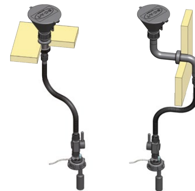
Figure 5 Schematic diagram of a funnel with a discharge pipe and level monitoring for installation in a fume cupboard. With a comprehensive approach at the planning stage, the proper handling of hazardous substances, as well as their storage and disposal, will be made easier for the later users of the laboratory.
