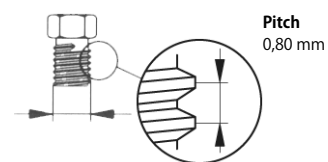
M 5 – outer- \varnothing = 5 mm
