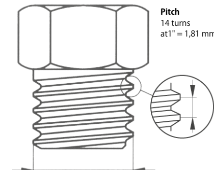
G 3/4" – outer-Ø = 26,3 mm
